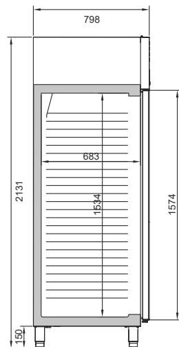
Parrillas reforzadas Reinforced wire shelves Grilles renforcées
